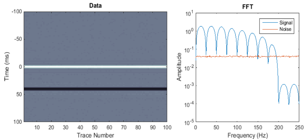
Figure 1 Synthetic data (left) and its amplitude spectra (right).
