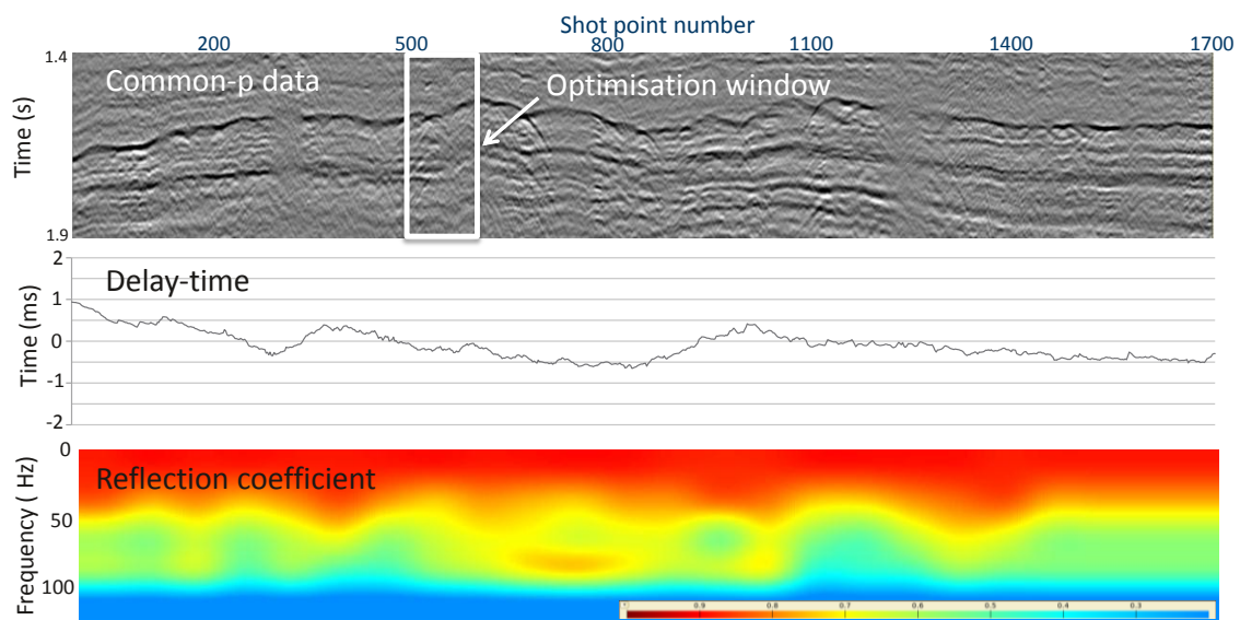
Figure 5 De-ghosted common- p section (top), estimated delay-time between primary and ghost (middle) and estimated reflection coefficient (bottom).
