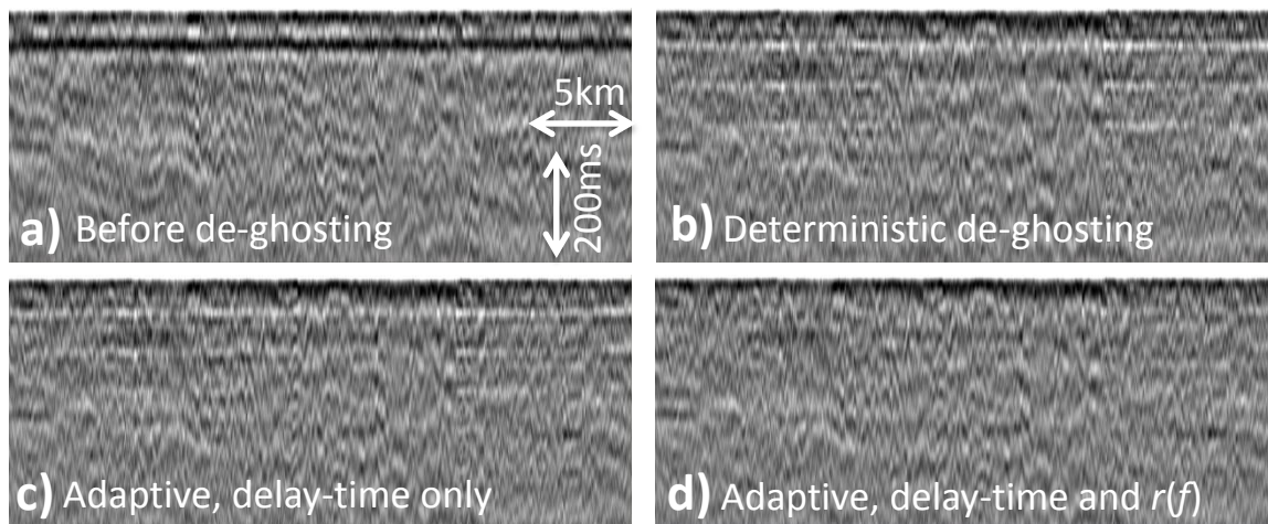
Figure 6 Autocorrelations of the common-p section in Figure 4. a) before de-ghosting, b) after deghosting with fixed parameters, c) after de-ghosting with optimized delay times and fixed reflection coefficient, d) after de-ghosting with optimized delay times and frequency-dependent reflection coefficient.
