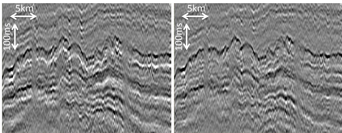
Figure 4 A common- p section before (left) and after (right) adaptive de-ghosting with optimized time delays and frequency-dependent reflection coefficient.
