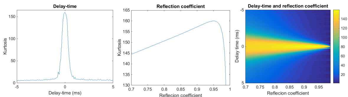
Figure 2 Objective function for ghost delay-time (left), reflection coefficient (middle) and joint optimisation (right).
